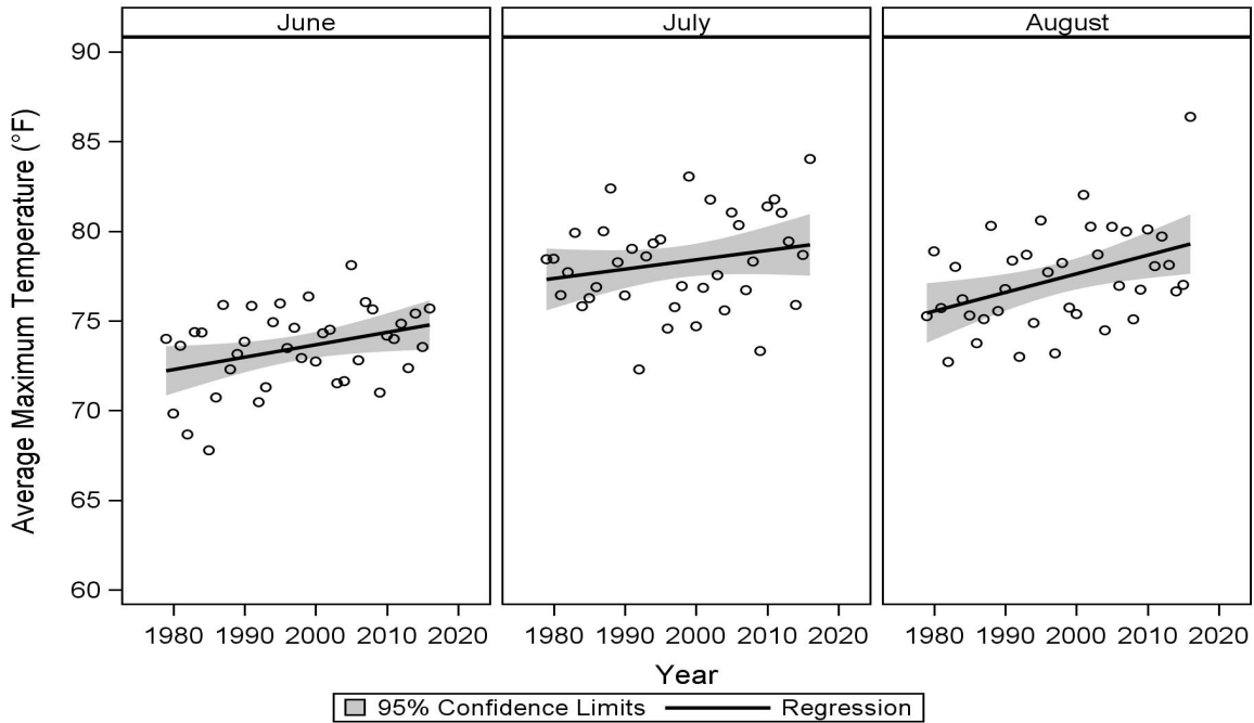
Figure 1c. Genesee County: Monthly Averages of Daily Maximum Temperature, 1979 - 2016
