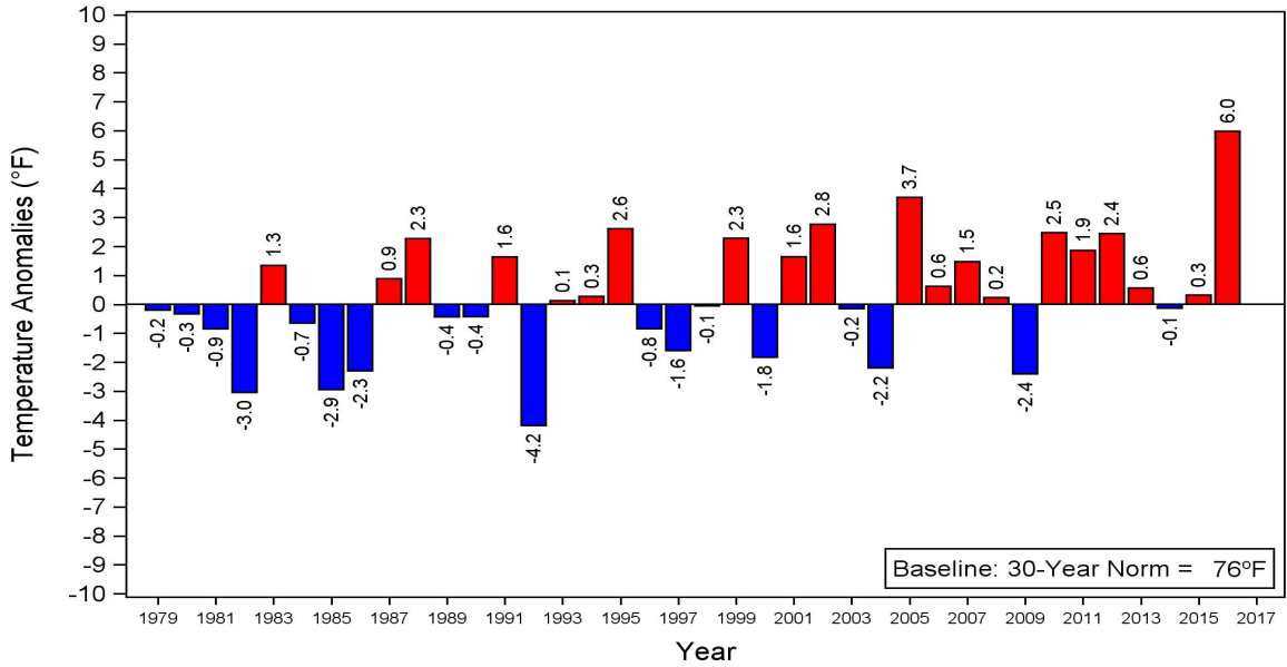
Figure 1b. Summer Temperature Anomalies in Genesee County, 1979 to 2016
